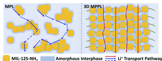
Fig. 10 Visual comparison of \text{Li}^+ transport in a random MOF–polymer blend (MPL, left) versus a well-aligned 3D MOF–polymer percolated layer (3D MPPL, right). Random distribution leads to discontinuous ionic pathways and increased resistance, while structured 3D architectures enable efficient, continuous \text{Li}^+ conduction. Adapted from ref. 91 with permission from AAAS, copyright 2023.
