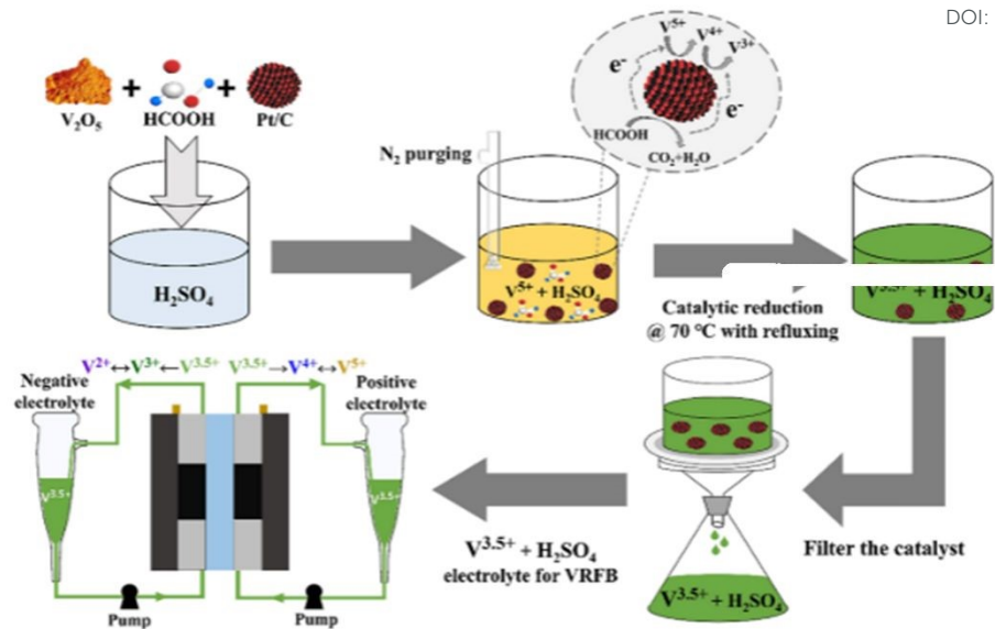
Fig. 8. Schematic of V^{3.5+} electrolyte preparation using hydrothermal reduction 16 (Reprinted with permission of American Chemical Society)
