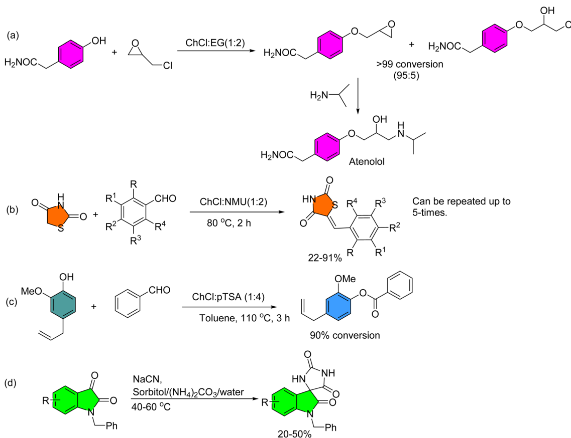
Fig. 3 (a) The synthesis of the drug Atenolol using a RNADES system. (b). The synthesis of thiazolidine-2,4-dione lipxygenase inhibitors with RNADES; NMU = N -methylurea. (c) Synthesis of eugenol benzoate using an acidic RNADES. (d) The use of a novel carbonate based RNADES for a Bucherer–Bergs multicomponent reaction.
