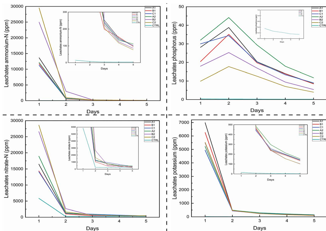
Fig. 5 Leachate concentrations showing continuous release of \text{NH}_4^+ / \text{NO}_3^- -N, P, and K above the control soil without BC amendment over the period of the experiment (inserted graphs scaled to show trend vividly).
