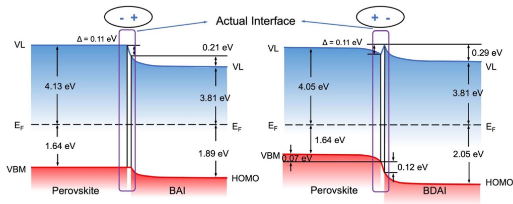
Fig. 4 Energy level diagram of the interface between perovskite and BAI/BDAl.
