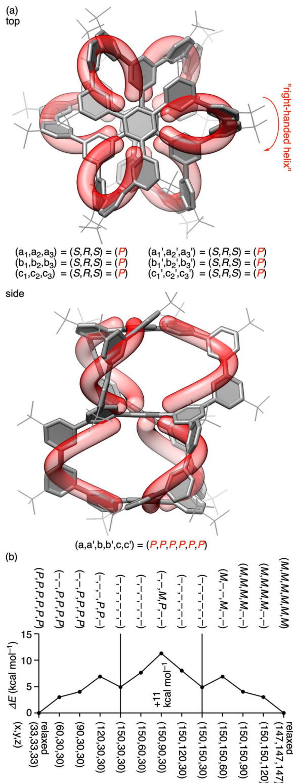
Fig. 4 Structure of phenine dipolluxene ( 1 ). (a) Crystal structure. A representative structure of the ( P,P,P,P,P,P )-isomer is shown. The mirror-image enantiomer, ( M,M,M,M,M,M ), was also found in the crystal of the racemate (Fig. S4). (b) Energetics of the conformers, showing an energy barrier of \sim 11 kcal mol -1 between the two enantiomers. Calculations were performed by using a methyl substituted molecule as a model. The helicity of the arms was assigned by adopting a system with ( S,R,S ) = ( P ) and ( R,S,R ) = ( M ), and conformations with other relationships were judged as non-helical and were described as “-”. See also Fig. S5.
