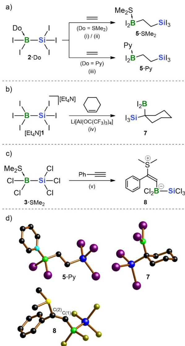
Scheme 2 (a) 1,2-Silaborations of ethylene with 2·SMe 2 or 2·Py afford 5·SMe 2 or 5·Py . (b) 1,1-Silaboration of cyclohexene with [Et 4 N] + 1 / Li[Al(OC(CF 3 ) 3 ) 4 ] furnishes 7 . (c) Reaction of phenylacetylene with 3·SMe 2 leads to the addition of the 3/SMe 2 Lewis pair across the C≡C bond to give 8 . (d) Solid-state structures of 5·Py , 7 , and 8 ; H atoms are omitted for clarity. Color code: B: green, C: black, N: pale blue, Si: blue, S: yellow, Cl: yellow-green; I: violet. Reagents and conditions: (i) exc. ethylene, CD 2 Cl 2 , 80 °C, 6 d, 98% yield; (ii) exc. ethylene, 0.1 eq. Bl 3 , CD 2 Cl 2 , rt, 12 h, 85% yield; (iii) exc. ethylene, oDFB, 120 °C, 20 d, 97% yield; (iv) 10 eq. cyclohexene, 1 eq. Li[Al(OC(CF 3 ) 3 ) 4 ] , oDFB, rt, 15 min, 99% yield; (v) 5 eq. phenylacetylene, CH 2 Cl 2 , rt, 1 d, 37% yield.
