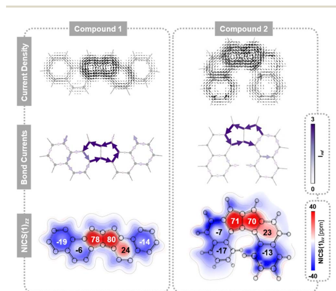
Fig. 2 Aromaticity comparison between 1 and 2 . (Top) current density plots generated with SYMOIC at a height of 1 Å above the molecular plane under a perpendicular magnetic field (only the contribution of the \pi -orbitals to the induced current density is taken into account). (Middle) net bond current strengths reported relative to the bond current strength of benzene. (Bottom) 2D NICS(1) zz plots (in ppm). The NICS(1) zz value of each ring is denoted within it.
