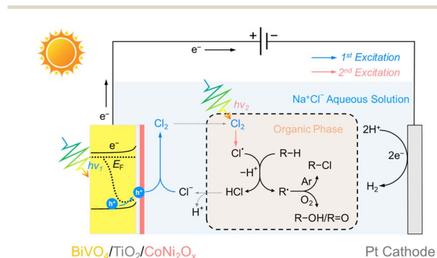
Scheme 2 Schematic illustration of the two-step coupled PEC C-H activation process. E_F is the quasi-Fermi level of the photoanode.
