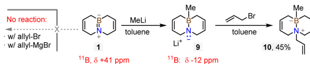
Scheme 3 Initial exploration of disrupting the B=N \pi -donation for double functionalization.
