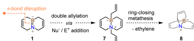
Scheme 2 The proposed double B=N allylation as a strategy towards a propellane core.
