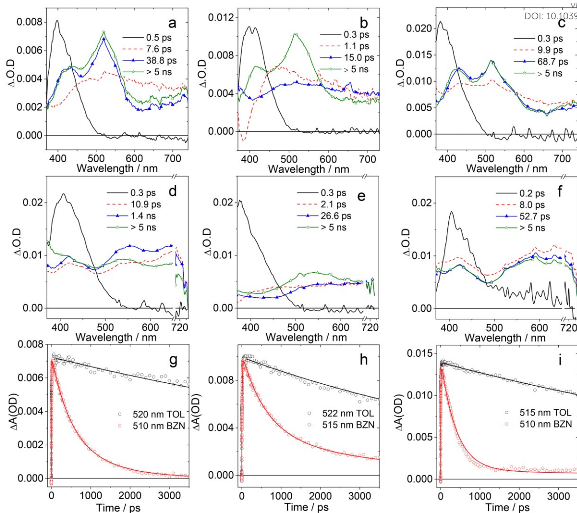
Fig. 5 EADS obtained from global analysis of the transient absorption data recorded for (a) PTZ-DTO , (b) PSeZ-DTO and (c) DPTZ-DTO in TOL upon excitation at 350 nm. Panels (g), (h) and (i) report a comparison of the kinetic trace recorded at the maximum of the \text{PTZ}^{+\bullet} signal for the three compounds in TOL and benzonitrile (BZN). Panels (d), (e) and (f) report the EADS obtained from global analysis of the transient absorption data recorded for (g) PTZ-O-DTO , (h) PTZ-O2-DTO and (i) DPTZ-O-DTO in TOL upon excitation at 350 nm.
