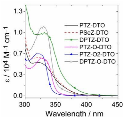
Fig. 1 UV/vis absorption spectra of the compounds in dichloromethane (DCM). c = 3.0 \times 10^{-4} M, 25 °C.
