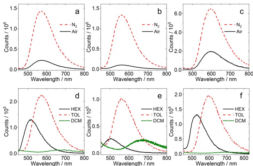
Fig. 2 Fluorescence emission spectra of the compounds under \text{N}_2 and air atmosphere of (a) PTZ-DTO , (b) PSeZ-DTO and (c) DPTZ-DTO in toluene (TOL). Fluorescence emission spectra of the compounds in different solvents of (d) PTZ-DTO , (e) PSeZ-DTO and (f) DPTZ-DTO in aerated solution. Optically-matched solutions were used, A = 0.1 , \lambda_{\text{ex}} = 310 nm, 25 °C.
