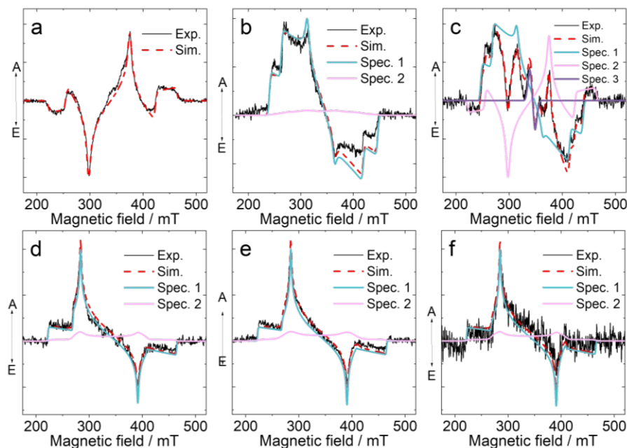
Fig. 8 Experimental (black) and simulated (red) TREPR spectra of (a) PTZ-DTO , (b) PSeZ-DTO , (c) DPTZ-DTO , (d) PTZ-O-DTO , (e) PTZ-O2-DTO and (f) DPTZ-O-DTO with parameters given in Table 5. The experimental spectra are shown for a 500 ns delay after the laser flash with an integration window of 100 ns. The laser excitation wavelength is 355 nm, c = 5.0 \times 10^{-4} M in solvents TOL/2MeTHF (3/1, v/v). Blue and purple color represent the decomposition of the experimental spectrum into two spectra with similar D , E parameters but multiplet and net polarizations, respectively. Three different triplet states were used in the simulation spectrum of DPTZ-DTO (see Table 5 for details). The spin-polarised patterns are characterised by absorptive (A) and emissive (E) features: positive features are in enhanced absorption (A) and negative features are in emission (E).
