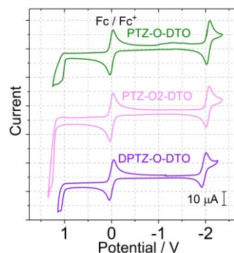
Fig. 4 Cyclic voltammograms of the compounds PTZ-O-DTO , PTZ-O2-DTO were studied in deaerated acetonitrile (ACN), DPTZ-O-DTO was studied in deaerated DCM. Ferrocene (Fc) was used as internal reference (set as 0 V in the cyclic voltammograms), 0.10 M Bu 4 NPF 6 as supporting electrolyte. Scan rates: 50 mV/s, c = 1.0 \times 10^{-4} M, 25 °C.
