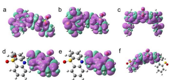
Fig. 10 Spin density surfaces of the dyads in the T_1 state of (a) PTZ-DTO , (b) PSeZ-DTO , (c) DPTZ-DTO , (d) PTZ-O-DTO , (e) PTZ-O2-DTO and (f) DPTZ-O-DTO in TOL, isovalue = 0.02. Calculations were performed with DFT at the B3LYP/6-31G(d) level with Gaussian 16.
