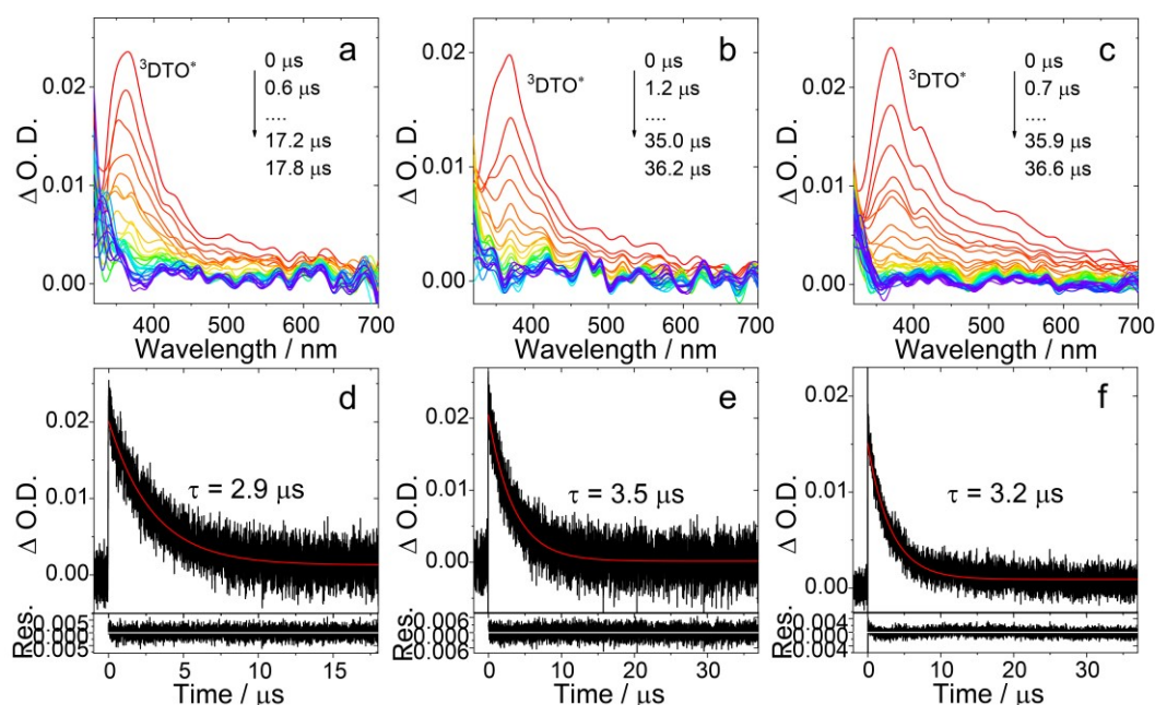
Fig. 7 Nanosecond transient absorption spectra of (a) PTZ-O-DTO , (b) PTZ-O2-DTO and (c) DPTZ-O-DTO . Decay curves of (d) PTZ-O-DTO , (e) PTZ-O2-DTO and (f) DPTZ-O-DTO at 370 nm after pulsed laser excitation at 355 nm. c = 2.0 \times 10^{-5} \text{ M} in deaerated TOL, 25 °C.
