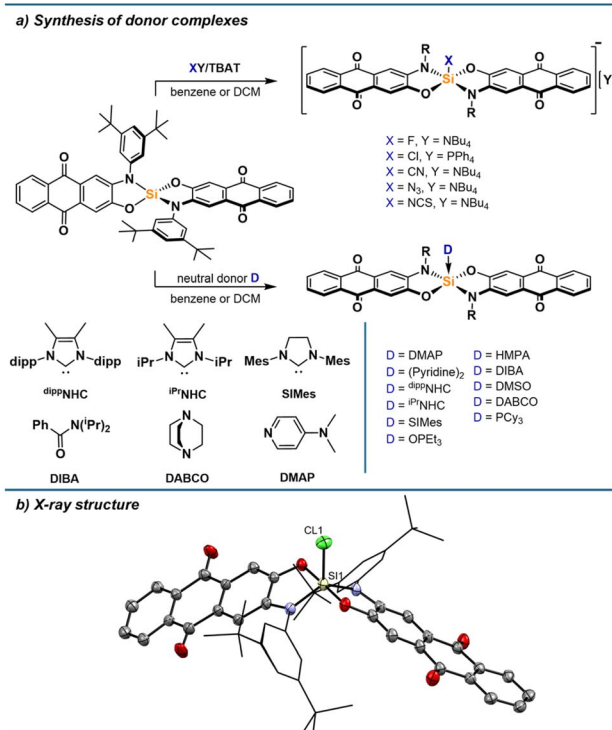
Fig. 5 (a) Synthesis of pentacoordinate silicon complexes with neutral and anionic donors. (b) Molecular structure of [1-Cl][PPh 4 ] determined by SCXRD analysis. Hydrogen atoms and the \text{PPh}_4 cation are omitted for clarity. Thermal displacement ellipsoids are displayed at the 50% probability level. Selected bond lengths [pm]: Si1–Cl1: 211.64(10), Si1–O1: 174.78(18), Si1–N1: 178.1(2). Selected bond angles [°]: N1–Si1–N1: 128.16(10), O1–Si1–O4: 177.74(9), N1–Si1–Cl1: 116.45(8), O1–Si1–Cl1: 91.53(7).
