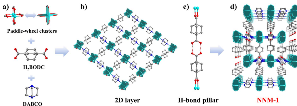
Fig. 1 The assembly and structure of NNM-1 : (a) three starting components for the assembly of NNM-1 ; (b) two-dimensional (4, 4)-squared layer; (c) hydrogen-bonded pillar (a pair of HBODC − ); (d) double-interpenetrated structure of NNM-1 . Color codes: Cu, sky blue; C, gray; H, white; O, red; and N, blue.
