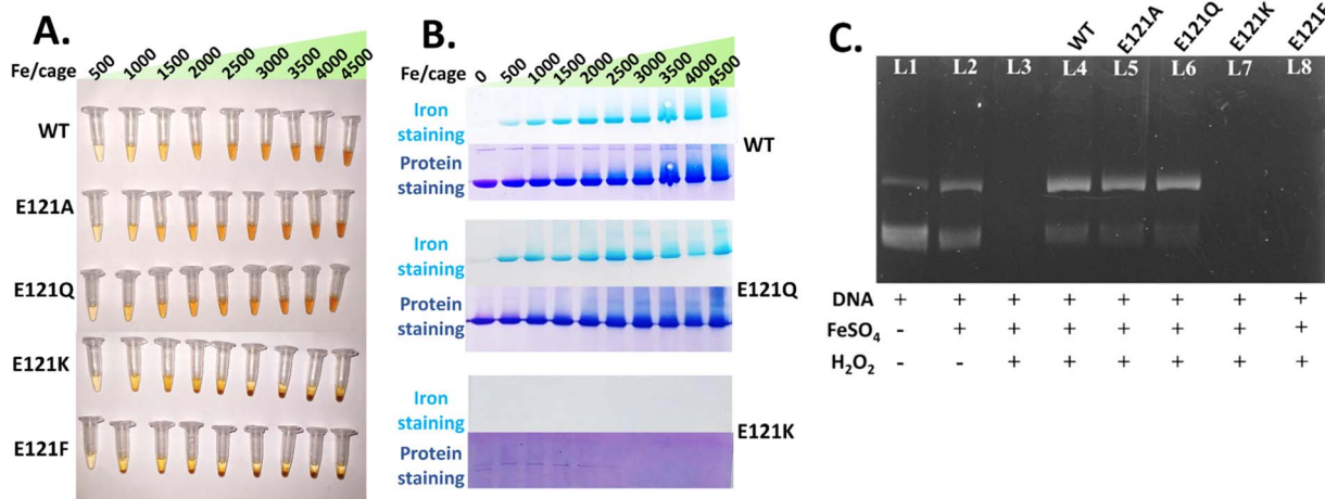
Fig. 5 Analysis of iron incorporation ability and DNA protection activity of Mtb BfrA variants. (A) The self-assembled variants hold iron in a soluble form almost up to the addition of 4500 Fe/cage whereas for the assembly-defective variants distinct precipitation was seen beyond 500 Fe/cage. (B) Native-PAGE analysis of iron loading efficiency/accumulation in assembled and assembly-defective variants. WT and E121Q exhibited similar behaviour with higher iron loading, but E121K showed a complete absence of Prussian Blue precipitate. The gradual disappearance of protein bands on increasing iron for E121K indicates iron-induced protein precipitation. Protein samples, with and without iron mineral incorporation, were run in a 6% (w/v) non-denaturing gel (native-PAGE) for checking the iron loading ability (top) and cage integrity (bottom). (C) DNA protection activity of WT Mtb BfrA and its 3-fold assembled variants against oxidative cleavage induced by the Fenton reaction. Agarose gel (0.8% w/v) electrophoresis was carried out to assess the DNA protection activity of Mtb BfrA and its self-assembled/assembly-defective variants. DNA protection was observed only for self-assembled variants (L4 to L6) whereas the assembly-defective variants (L7 and L8) could not provide protection. For the control experiment: L1: only DNA; L2: iron and DNA; L3: DNA, iron and H 2 O 2 (the absence of DNA bands indicates oxidative cleavage). ± signs represent the presence/absence of DNA, H 2 O 2 and Fe 2+ ions.
