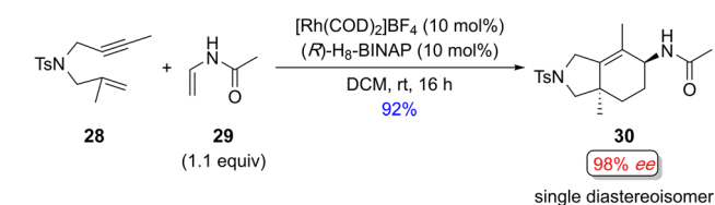
Scheme 17 Representative example of a diastereo- and enantioselective Rh(I)-catalyzed [(2+2)+2] of a 1,6-enyne with an exogenous enamide.
