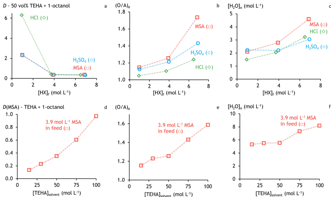
Fig. 4 Solvent extraction data of \text{H}_2\text{SO}_4 , HCl, and MSA – TEHA + 1-octanol systems at 25 °C. Systems depicted in a to c contain 50 vol% TEHA in 1-octanol, and in d to f contain a variable amount of TEHA in 1-octanol. Distribution ratios (a and d), volume changes (b and e), and water uptake by the solvent (c and f) are shown.
