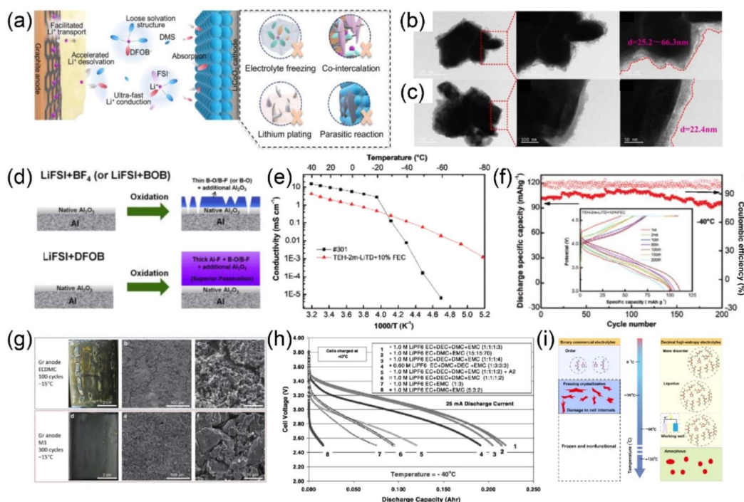
Fig. 5 (a) Advantages of mixed lithium salts in electrolytes. Based on ref. 90. (b and c) TEM analysis of various electrolytes following 50 cycles at -40^{\circ}\text{C} . Based on ref. 91. (d) Schematic diagram of forming passivation film on aluminum electrode using electrolytes of different lithium salts. Based on ref. 92. (e) Comparison of electrolyte conductivity at various temperatures. (f) Electrochemical performance of Li||NCM523 battery at -40^{\circ}\text{C} when charged to 4.6 V with current density of 1C. Based on ref. 93. (g) Optical and SEM images at the graphite anode at -15^{\circ}\text{C} . Based on ref. 58. (h) -40^{\circ}\text{C} , discharge capacity of batteries with different carbonate based electrolyte. Based on ref. 94. (i) Schematic diagram of the change of commercial binary and designed decimal high entropy electrolyte with temperature decreasing. Based on ref. 95.
