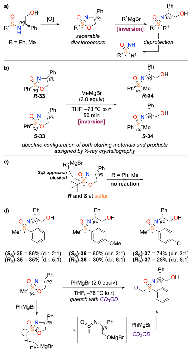
Scheme 9 (a) Route to access enantioenriched sulfoximines via cyclic sulfonylimides; (b) reaction between cyclic sulfonylimides and methyl magnesium bromide, unequivocally proving inversion at the sulfur centre by X-ray crystallography; (c) steric bulk of tert -butyl cyclic sulfonylimides potentially blocking the \text{S}_{\text{N}}2 trajectory of Grignard nucleophiles; (d) erosion of enantiopurity at the sulfur stereocentre via proposed sulfene intermediate.
