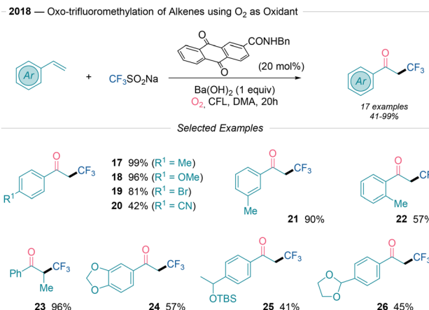
Scheme 4 Photoredox synthesis of α-trifluoromethylketones reported by Itoh. 21
