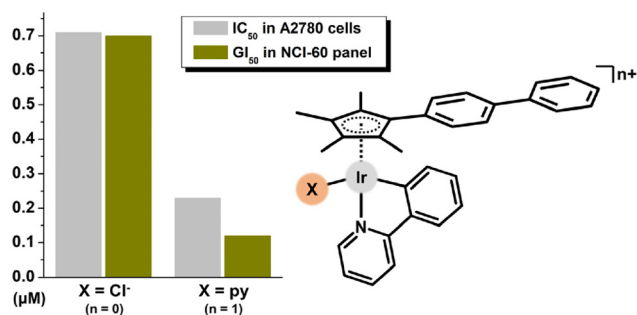
Fig. 35 A comparison of the in vitro antiproliferative activity of [\text{Ir}(\eta^5\text{-Cp}^{\text{pph}})(\text{ppy})(\text{X})]^{n+} complexes containing different monodentate ligands ( \text{X} = \text{Cl} and n = 0 for 47 ; \text{X} = \text{py} and n = 1 for 101 ).
