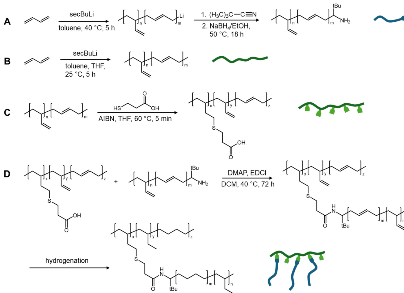
Fig. 1 Reaction scheme of (A) amine-terminated 1,4-PB, n/(m+n) = 0.12 ; (B) 1,2-PB, n/(m+n) = 0.89 ; (C) carboxyl functionalized 1,2-PB, and (D) poly(ethylene- g -polyethylene).
