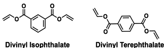
Fig. 9 Structures of divinyl isophthalate and divinyl terephthalate.
