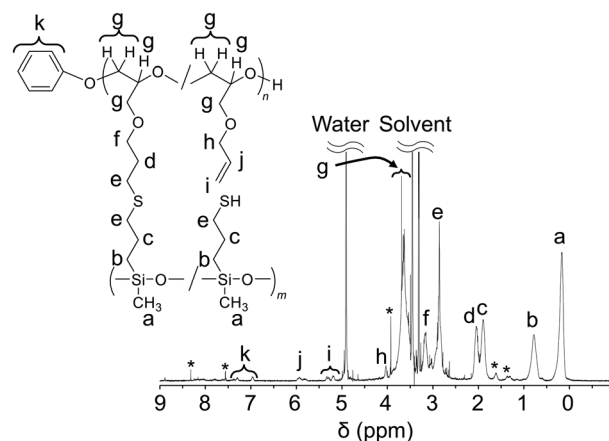
Fig. 2 1 H NMR spectrum of PGE-PAMS in CD 3 OD. The chemical shifts are referenced to CD 3 OD ( \delta 3.31). *: Unknown signal.
