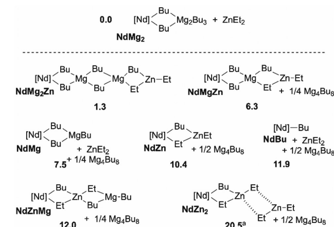
Scheme 3 Speciation of the alkylated species yielded from [\text{Nd}](\mu\text{-}^n\text{Bu})_2\text{-Mg}_2^{\text{n}}\text{Bu}_3 and \text{ZnEt}_2 . Only the most stable species are shown, the fully detailed speciation is provided in ESI.† \Delta G in kcal mol -1 . a In NdZn 2 , interaction between the \text{ZnEt}_2 fragments is weak, the endergonicity results from the entropy cost of the association of free and separated \text{ZnEt}_2 . Gaussian 09, B3PW91/D3BJ(SP), SMD(TolH), 298 K, 1 atm.
