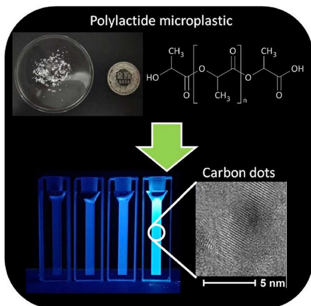
Fig. 7 Illustration of synthesizing fluorescent CDs from PLA with a hydrothermal method, which can be excited with UV light. The crystalline structure of a single CD is shown at the right corner. Reprinted with permission from ref. 61. Copyright 2020 Elsevier.
