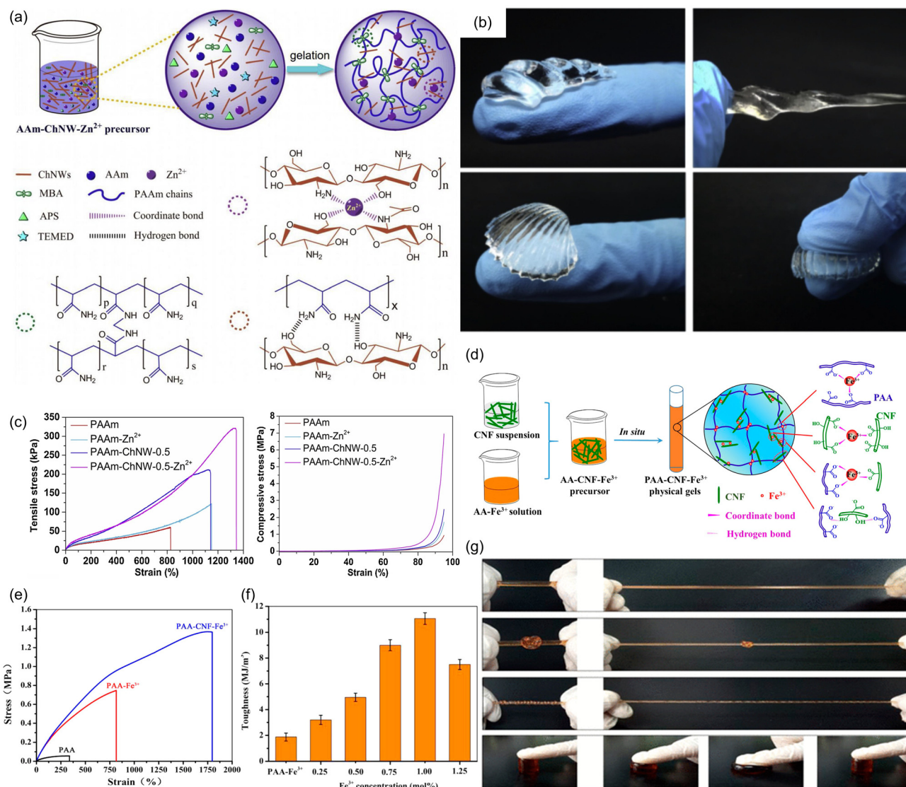
Fig. 25 Mechanical properties of hydrogels enhanced by metal coordination sacrificial bonds. (a) Scheme showing polyacrylamide gels with chitin nanowhiskers and \text{Zn}^{2+} ions (PAAm-ChNW- \text{Zn}^{2+} ). (b) Different shapes of PAAm-ChNW- \text{Zn}^{2+} achieved by twisting and bending. (c) Tensile and compressive stress versus strain curves of PAAm-ChNW- \text{Zn}^{2+} gels show that addition of \text{Zn}^{2+} increases both tensile strength and toughness. Reprinted from ref. 125 with permission from Elsevier, copyright 2020. (d) Scheme showing the formation of a PAA matrix with cellulose nanofibrils and \text{Fe}^{3+} ions (PAA-CNF- \text{Fe}^{3+} ). (e) Uniaxial tensile tests reveal enhancement of mechanical properties upon addition of CNF and \text{Fe}^{3+} ions. (f) Tensile toughness varies with [\text{Fe}^{3+}] in PAA-CNF- \text{Fe}^{3+} . (g) PAA-CNF- \text{Fe}^{3+} gels can be (from top) stretched, knotted, twisted and compressed. Adapted with permission from ref. 126. Copyright 2017 American Chemical Society.
