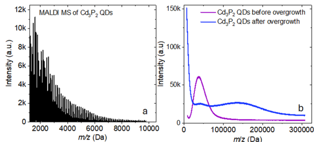
Fig. 5 (a) MALDI MS of Cd 3 P 2 QDs emitting at 1010 nm in the low-mass region before cluster overgrowth. (b) MALDI MS of Cd 3 P 2 QDs in the high-mass region before and after cluster overgrowth.
