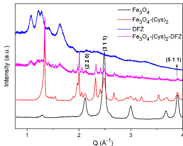
Fig. 8 X-ray powder diffraction patterns of \text{Fe}_3\text{O}_4 (black line), \text{Fe}_3\text{O}_4 -(Cys) 2 (red line), \text{Fe}_3\text{O}_4 -(Cys) 2 -DFZ (magenta line) and DFZ (blue line). The diffractograms were normalized by the maximum peak intensity and vertically displaced for better visualization.
