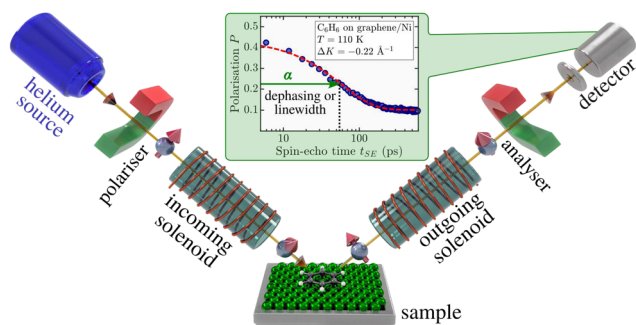
Fig. 4 Schematic of a helium spin-echo (HeSE) apparatus. The spin of the 3 He atoms acts as an internal timer that can be manipulated by magnetic solenoids before and after scattering. The interference of two time-separated wave packets allows detection of surface motion via a change in spin-polarisation upon scattering from the moving adsorbates. The inset shows a typical intermediate scattering function (ISF, I(\Delta K, t_{SE}) ), reflecting the time-dependent correlation of the adsorbate dynamics via measurement of the quasi-elastic linewidth or dephasing rate \alpha .
