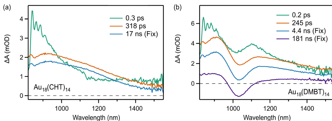
Fig. 3 Global analysis of fs-TA data of (a) \text{Au}_{18}(\text{CHO})_{14} and (b) \text{Au}_{18}(\text{DMBT})_{14} in the NIR region.
