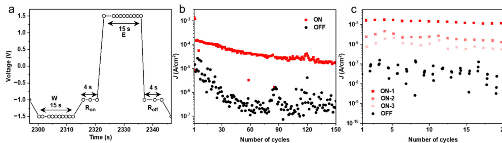
Fig. 5 Switching of the junctions. (a) the WRED pulse sequence, (b) the endurance over 150 WRED cycles, (c) the output current of the dynamic junction.
