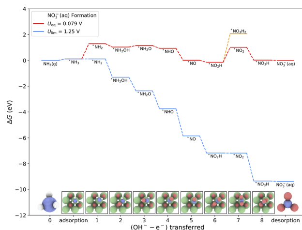
Fig. 14 Free energy diagram for \text{NO}_3^-(\text{aq}) formation by proceeding through the same mechanistic steps towards \text{NO}_2^-(\text{aq}) . After \text{*NO}_2\text{H} is formed, the mechanism branches towards \text{*NO}_2 or \text{*NO}_3\text{H}_2 , with the deprotonation step being energetically preferred. The energy required for the final desorption step was calculated to be -0.029 eV. Equilibrium (red trace) and limiting (blue trace) potentials are calculated using the computational hydrogen electrode at pH 11.
