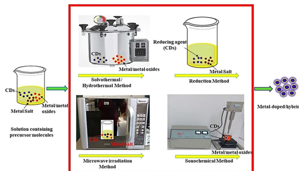
Fig. 6 Schematic representation of various methods used for synthesizing the metal-doped and hybrid CDs. Reproduced with permission. 79 Copyright 2025, Elsevier.
