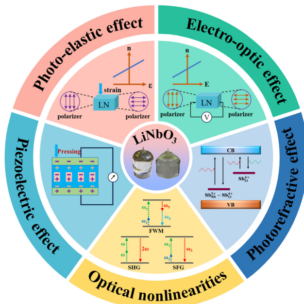
Fig. 1 Properties of LiNbO 3 crystals.
