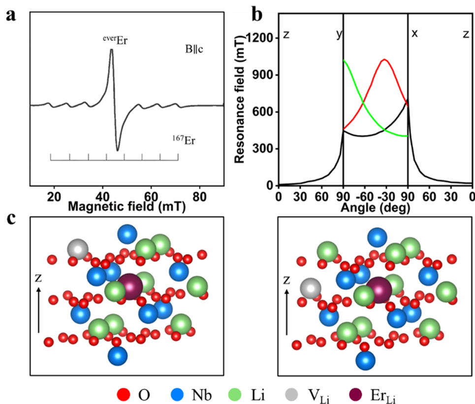
Fig. 9 (a) EPR spectrum of \text{Er}^{3+} in \text{LiNbO}_3 , measured at T = 5 \text{ K} and \nu_{\text{EPR}} = 25 \text{ GHz} . 130 Reproduced from ref. 130 with permission from Elsevier, copyright 1997. (b) Angular dependence of the EPR spectra of the \text{LN}:\text{Er}^{3+} crystal measured at 8 \text{ K} in all three perpendicular planes. 128 Reproduced from ref. 128 with permission from John Wiley and Sons, copyright 2008. (c) Possible models of low-symmetry \text{Er}^{3+} centers. 131 Reproduced from ref. 131 with permission from Materials Research Society, copyright 2009.
