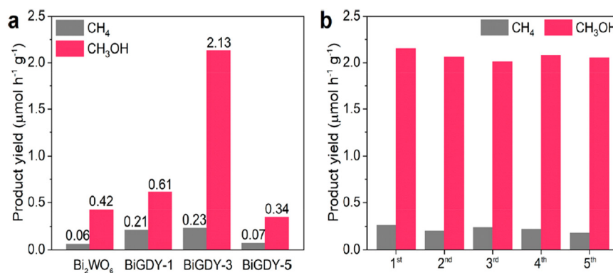
Fig. 9 (a) Photocatalytic \text{CO}_2 reduction performance of samples. (b) Cycling tests of the GDY/ \text{Bi}_2\text{WO}_6 heterojunction (BiGDY). Reproduced with permission from ref. 139. Copyright 2021, American Chemical Society.
