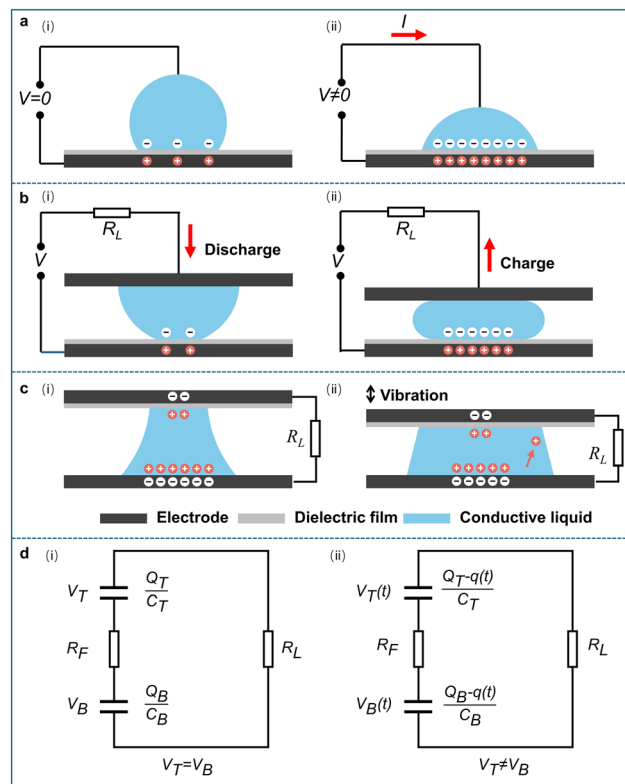
Fig. 3 Basic working principles and equivalent circuit diagram. a) Working principle of the EWOD process. (i) No external voltage applied between the metal and the electrolyte solution; (ii) external voltage applied between the metal and the electrolyte solution. b) Working principle of the REWOD process. c) Working principle of the water bridge REWOD process. d) Equivalent circuit diagram of the water bridge REWOD process.
