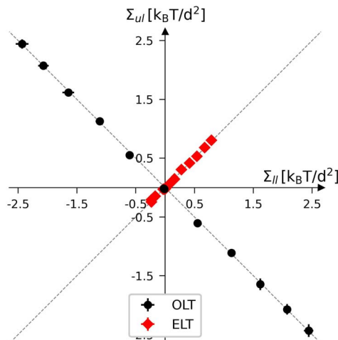
Fig. 3 Leaflet tension space for planar bilayers that contain a total number of N_{||} + N_{ul} = 1682 lipids. 18 The two coordinates are the leaflet tensions \Sigma_{||} and \Sigma_{ul} in the lower and upper leaflets. Negative and positive leaflet tensions describe compressed and stretched leaflets. The reference state with tensionless leaflets, corresponding to \Sigma_{||} = \Sigma_{ul} = 0 , is obtained for the symmetric bilayer with N_{||} = N_{ul} = 841 lipids. The red data points describe elastic deformations with equal leaflet tensions (ELTs), \Sigma_{||} = \Sigma_{ul} . The black data points represent bilayers with opposite leaflet tensions (OLTs), \Sigma_{||} = -\Sigma_{ul} and \Sigma = 0 . All OLT states can be obtained from the reference state by reshuffling lipids from one leaflet to the other and adjusting the base area of the simulation box to obtain tensionless bilayers.
