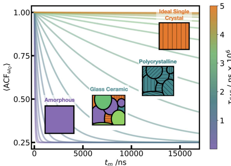
Fig. 7 Schematic of range of crystalline to amorphous \tau_{SAE} . The plot shows a range of decay functions, eqn (5), with \tau_{SAE} from 50 ns to 5 million ns. The inset figures show schematics of the expected microscale structure at each of these varying decay rates, with black lines in the glass ceramic and polycrystalline denoting different grains.
