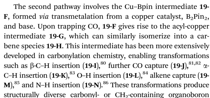
In the past five years, Wu and co-workers have reported a series of copper-catalyzed carbonylation reactions involving carbene
