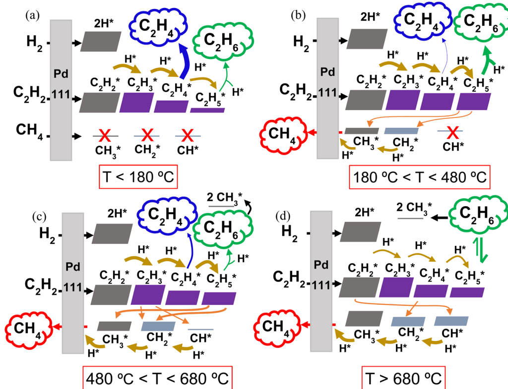
Fig. 5 Reaction pathway diagrams illustrating the reactions between the gaseous reactants ( C_2H_2 , H_2 and CH_4 ) and the catalyst surface (a) below 180^\circ\text{C} , (b) between 180 and 480^\circ\text{C} , (c) between 480 and 680^\circ\text{C} and (d) above 680^\circ\text{C} . The resulting adsorbed surface species (marked with * ) and their reactions with other surface species are also shown. The eventual desorption of the C_2H_4 (blue), C_2H_6 (green) and CH_4 (red) products (with varying concentrations depending on the temperature) is indicated by the cloud-shaped text boxes. Adsorption reactions are indicated by black arrows, surface hydrogenation reactions by mustard arrows, and surface dissociation reactions by orange arrows. The thickness of the arrows and the size of the blocks are qualitatively representative of the reaction rates and species surface coverage, respectively.
