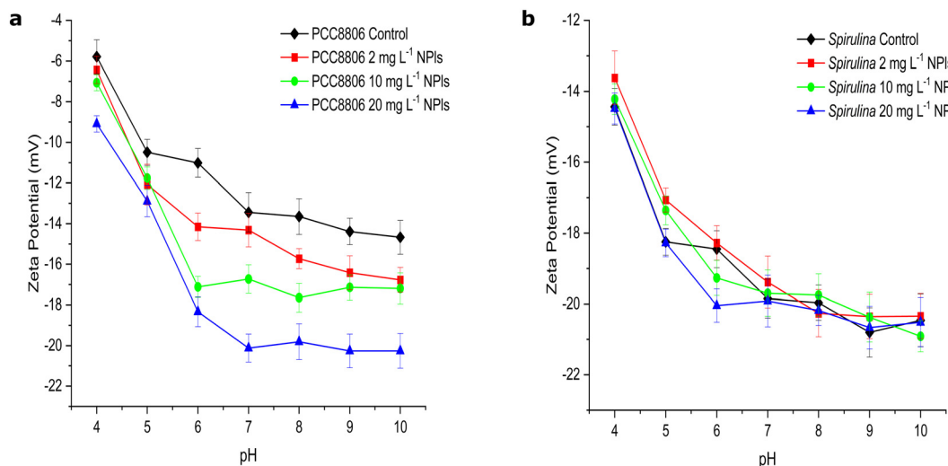
Fig. 3 Surface charge of PCC8806 and Spirulina under PS NPI exposure. Effects of PS NPIs on the ZPs of a. PCC8806 and b. Spirulina cells at the exponential phase in 0.1 M NaNO 3 at pH 4–10. Values are shown as mean \pm SD, n = 15 . Statistical significance is defined as p < 0.05 .
