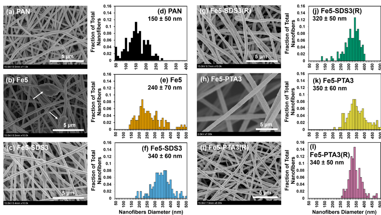
Fig. 1 SEM images (a–c and g–i) and histograms of nanofiber diameters (d–f and j–l; as measured by SEM image processing in ImageJ) for PAN, Fe5, Fe5–SDS3, Fe5–SDS3(R), Fe5–PTA3, and Fe5–PTA3(R). The Fe oxide particles obtained from vendor B were used for all of these materials. Average nanofiber diameters and standard deviation were determined by measuring at least n = 150 nanofibers for each material.
