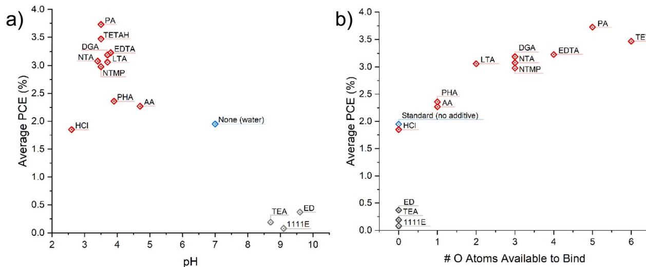
Fig. 5 Correlation of (a) the pH and (b) the number of potential Sb-binding O atoms of an additive employed in Sb 2 S 3 solar cells, and the performance of that additive in a solar cell. The additives used were none (standard), ethylenediaminetetraacetic acid (EDTA), pentetic acid (PA), triethylenetetramine- N,N,N',N'',N''',N''' -hexaacetic acid (TETAH), nitrilotriacetic acid (NTA), diglycolic acid (DGA), L-(+)-tartaric acid (LTA), nitrilotris(methylenephosphonic) acid (NTMP), phosphoric acid (PHA), acetic acid (AA), hydrochloric acid (HCl), triethanolamine (TEA), ethylenediamine (ED) and 1,1',1'',1'''-(ethane-1,2-diylbis(azanetriyl))tetrakis(propan-2-ol) (1111E). Reproduced from ref. 59 with permission from Royal Society of Chemistry, copyright 2025.
