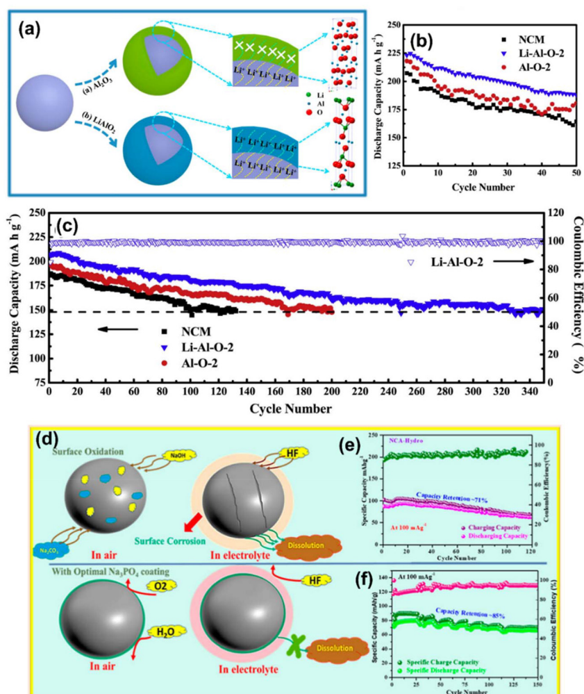
Fig. 44 (a) Schematic of coatings on NCM, (b) cycle performance of NCM, Al-O-2, and Li-Al-O-2 at 0.2\text{C} in a voltage range of 2.7\text{--}4.7 \text{ V}_{\text{Li/Li}^+} , (c) comparison of cycle performance of NCM, Al-O-2, and Li-Al-O-2 with an electrochemical window of 2.7\text{--}4.5 \text{ V}_{\text{Li/Li}^+} . 133 Copyright: 2018 Elsevier. (d) Schematic representation of \text{Na}_3\text{PO}_4 protection layer regarding surface corrosion. Cycling performance of (e) pristine Na-NCA, (f) \text{Na}_3\text{PO}_4@0.5 cathode at 100 \text{ mA g}^{-1} current density. 134 Copyright: 2024 American Chemical Society.
