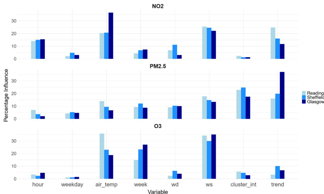
Fig. 7 Influence of explanatory variables and trend used by the deweather package when building statistical models of \text{NO}_2 , \text{PM}_{2.5} and \text{O}_3 for Reading, Sheffield and Glasgow. Variable "hour" refers to hour of day, "weekday" to day of week, "week" to week of year, "wd" to wind direction, "ws" to wind speed and "cluster_int" refers to the air mass back trajectory clusters in Fig. 6. Full PDs shown in Fig. S27–S29.†
