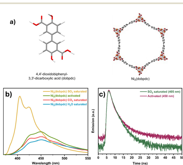
Fig. 10 (a) Structure of linker and \text{Ni}_2(\text{dobpdc}) , (b) selective response of \text{Ni}_2(\text{dobpdc}) towards \text{SO}_2 , and (c) decay-time of activated and \text{SO}_2 saturated samples (reproduced from ref. 67).
