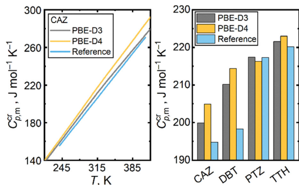
Fig. 6 Illustration of the temperature trends of experimental isobaric heat capacities C_{p,T}^r for crystalline carbazole and those calculated using the quasi-harmonic protocol and PBE-D3 and PBE-D4 models (left); and a comparison of experimental and calculated crystal-phase heat capacities at 298.15 K and ambient pressure for all the target materials (right).
