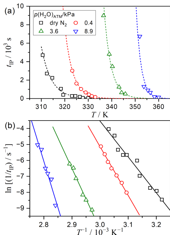
Fig. 2 Results of the conventional kinetic analysis for the IP process of the thermal dehydration of SC-MH under isothermal conditions in a stream of dry or wet N_2 with different p(H_2O)_{ATM} values, conducted using the fundamental kinetic equation (eqn (2)): (a) t_{IP} values at varying temperatures and p(H_2O)_{ATM} values and (b) Arrhenius-type plots for the IP process at individual p(H_2O)_{ATM} values. The dashed lines in (a) represent the replication curve, which was calculated using the results of the Arrhenius-type plots shown in (b).
