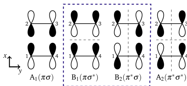
Fig. 2 Schematic of the four principal orbitals, with only carbons 1–4 and their p_x orbitals shown ( cf. Fig. 1). In NBD, the B_1 and B_2 orbitals are the HOMO and LUMO, respectively, and vice versa in QC. Inter-nuclear nodes are drawn as dashed lines. All four orbitals constitute the (4,4) active space, while the dashed box denotes the (2,2) active space. Orbitals from electronic structure calculations are shown in Section S1 of the ESI.†
