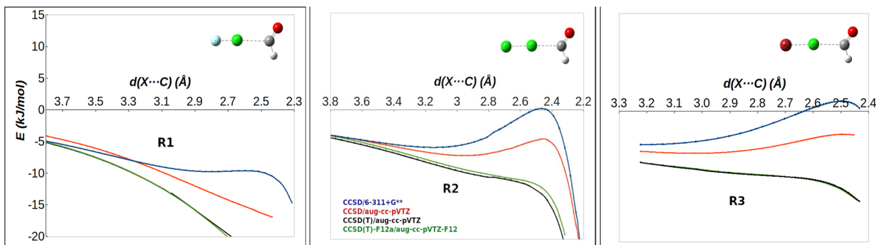
Fig. 5 PECs of reactions (R1) (left), (R2) (center) and (R3) (right) as obtained at the following levels of theory: CCSD/6-311+G(d,p) (in blue), CCSD/aug-cc-pVTZ (in red), CCSD(T)/aug-cc-pVTZ (in black) and CCSD(T)-F12a/aug-cc-pVTZ-F12 (in green). The corresponding TS structures are shown.
